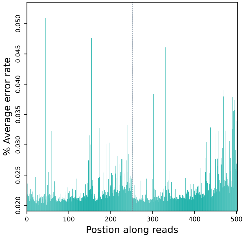
Error rate distribution along reads (R10220)
